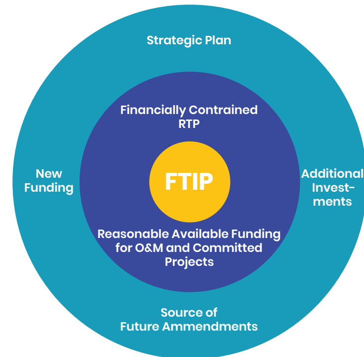
FIGURE 1 RTP Framework
